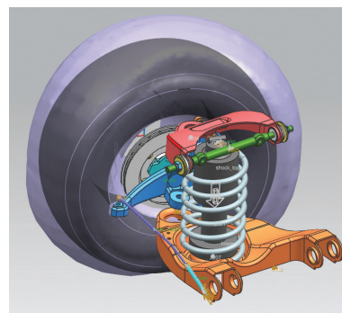
Create motion envelopes to design for package space and check for interference.
