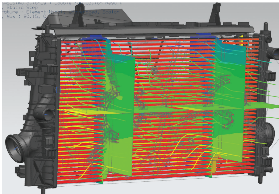
Hex mesh throughout central volume of geometry.
